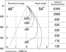
■ Direct Horizontal Illuminance DD155-1555DW9027-FX
