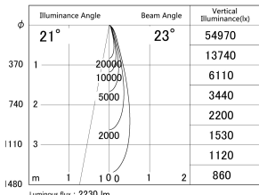
■ Direct Horizontal Illuminance DD155-2025DW9027-FX
