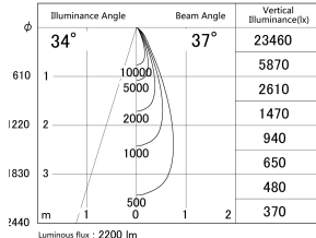
■ Direct Horizontal Illuminance DD155-2035DW9027-FX
