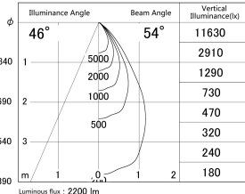
■ Direct Horizontal Illuminance DD155-2055DW9027-FX
