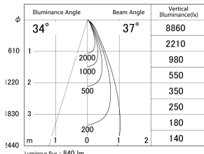
■ Direct Horizontal Illuminance DD155-0835DW9030-FX
