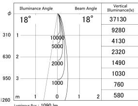
■ Direct Horizontal Illuminance DD155-1015DW9030-FX
