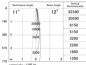
■ Direct Horizontal Illuminance DD155-1510DW9030-FX
