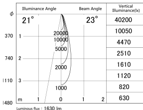
■ Direct Horizontal Illuminance DD155-1525DW9030-FX
