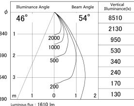
■ Direct Horizontal Illuminance DD155-1555DW9030-FX
