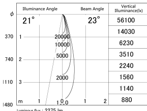
■ Direct Horizontal Illuminance DD155-2025DW9030-FX
