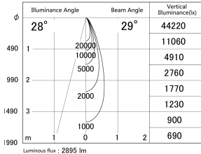
■ Direct Horizontal Illuminance DD155-2530DW9030-FX
