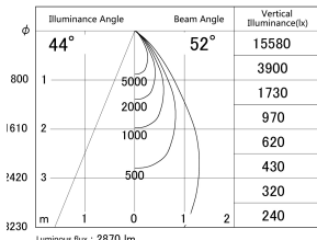
■ Direct Horizontal Illuminance DD155-2555DW9030-FX
