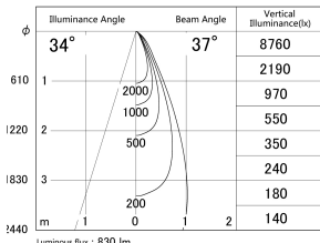
■ Direct Horizontal Illuminance DD155-0835DW9035-FX
