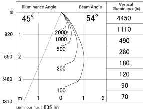
■ Direct Horizontal Illuminance DD155-0855DW9035-FX
