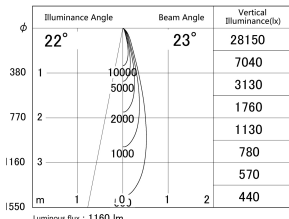
■ Direct Horizontal Illuminance DD155-1025DW9035-FX
