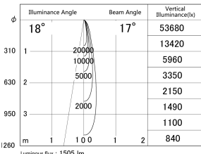
■ Direct Horizontal Illuminance DD155-1515DW9035-FX
