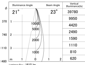
■ Direct Horizontal Illuminance DD155-1525DW9035-FX
