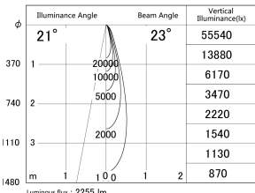
■ Direct Horizontal Illuminance DD155-2025DW9035-FX
