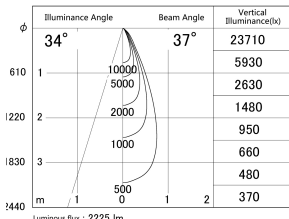
■ Direct Horizontal Illuminance DD155-2035DW9035-FX
