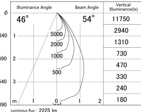
■ Direct Horizontal Illuminance DD155-2055DW9035-FX
