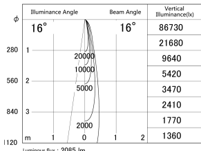
■ Direct Horizontal Illuminance DD155-2515DW9035-FX
