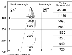
■ Direct Horizontal Illuminance DD155-2525DW9035-FX
