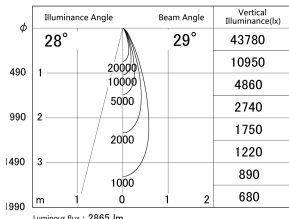
■ Direct Horizontal Illuminance DD155-2530DW9035-FX
