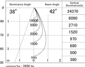
■ Direct Horizontal Illuminance DD155-2540DW9035-FX
