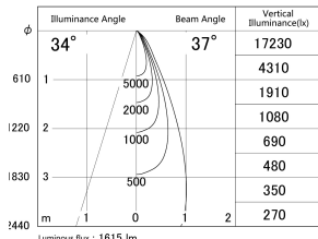
■ Direct Horizontal Illuminance DD155-1535DW9040-FX
