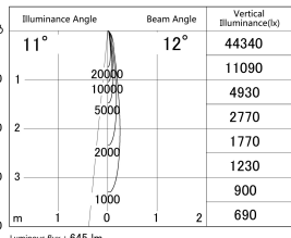
■ Direct Horizontal Illuminance DD155-0810DB9027-FX
