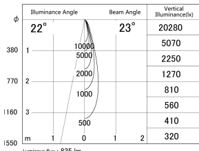
■ Direct Horizontal Illuminance DD155-0825DB9027-FX
