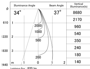
■ Direct Horizontal Illuminance DD155-0835DB9027-FX
