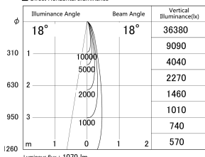
■ Direct Horizontal Illuminance DD155-1015DB9027-FX
