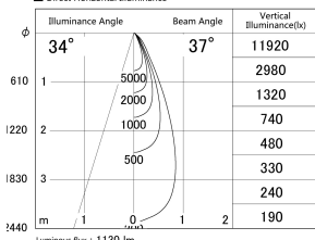
■ Direct Horizontal Illuminance DD155-1035DB9027-FX
