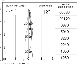
■ Direct Horizontal Illuminance DD155-1510DB9027-FX
