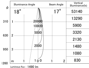
■ Direct Horizontal Illuminance DD155-1515DB9027-FX
