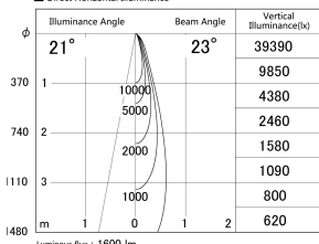
■ Direct Horizontal Illuminance DD155-1525DB9027-FX
