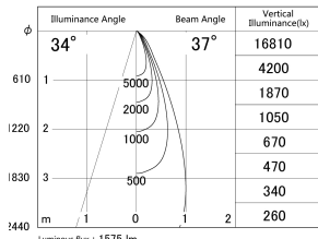
■ Direct Horizontal Illuminance DD155-1535DB9027-FX
