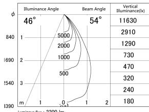
■ Direct Horizontal Illuminance DD155-2055DB9027-FX
