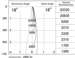
■ Direct Horizontal Illuminance DD155-2515DB9027-FX
