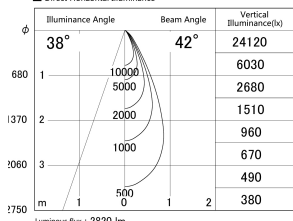
■ Direct Horizontal Illuminance DD155-2540DB9027-FX
