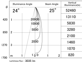
■ Direct Horizontal Illuminance DD155-3025DB9027-FX
