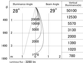
■ Direct Horizontal Illuminance DD155-3030DB9027-FX
