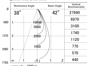
■ Direct Horizontal Illuminance DD155-3040DB9027-FX
