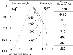
■ Direct Horizontal Illuminance DD155-3055DB9027-FX
