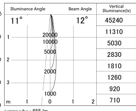
■ Direct Horizontal Illuminance DD155-0810DB9030-FX
