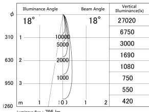
■ Direct Horizontal Illuminance DD155-0815DB9030-FX
