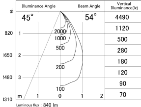
■ Direct Horizontal Illuminance DD155-0855DB9030-FX
