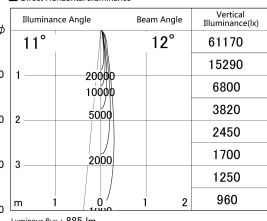
■ Direct Horizontal Illuminance DD155-1010DB9030-FX
