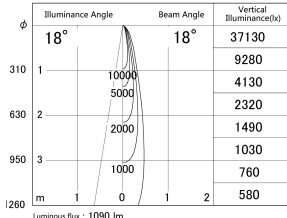
■ Direct Horizontal Illuminance DD155-1015DB9030-FX
