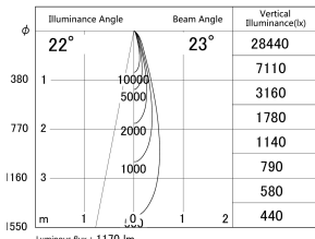
■ Direct Horizontal Illuminance DD155-1025DB9030-FX
