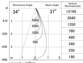
■ Direct Horizontal Illuminance DD155-1035DB9030-FX
