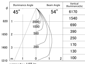
■ Direct Horizontal Illuminance DD155-1055DB9030-FX
