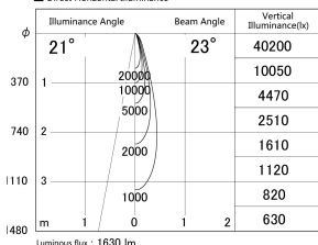
■ Direct Horizontal Illuminance DD155-1525DB9030-FX
